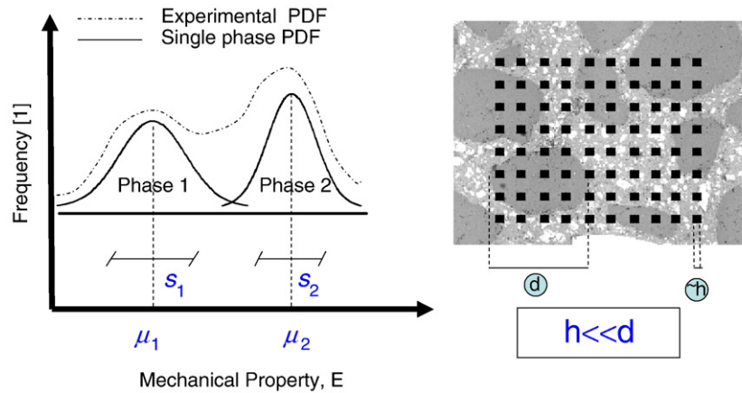
Fig. 5. Schematic representation of the deconvolution techniques for composite materials.
